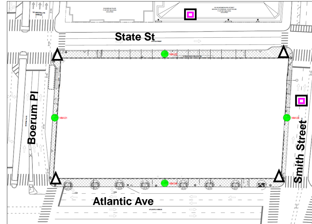
Vibration, Air and Noise monitoring devices installed by Design-Build team.
