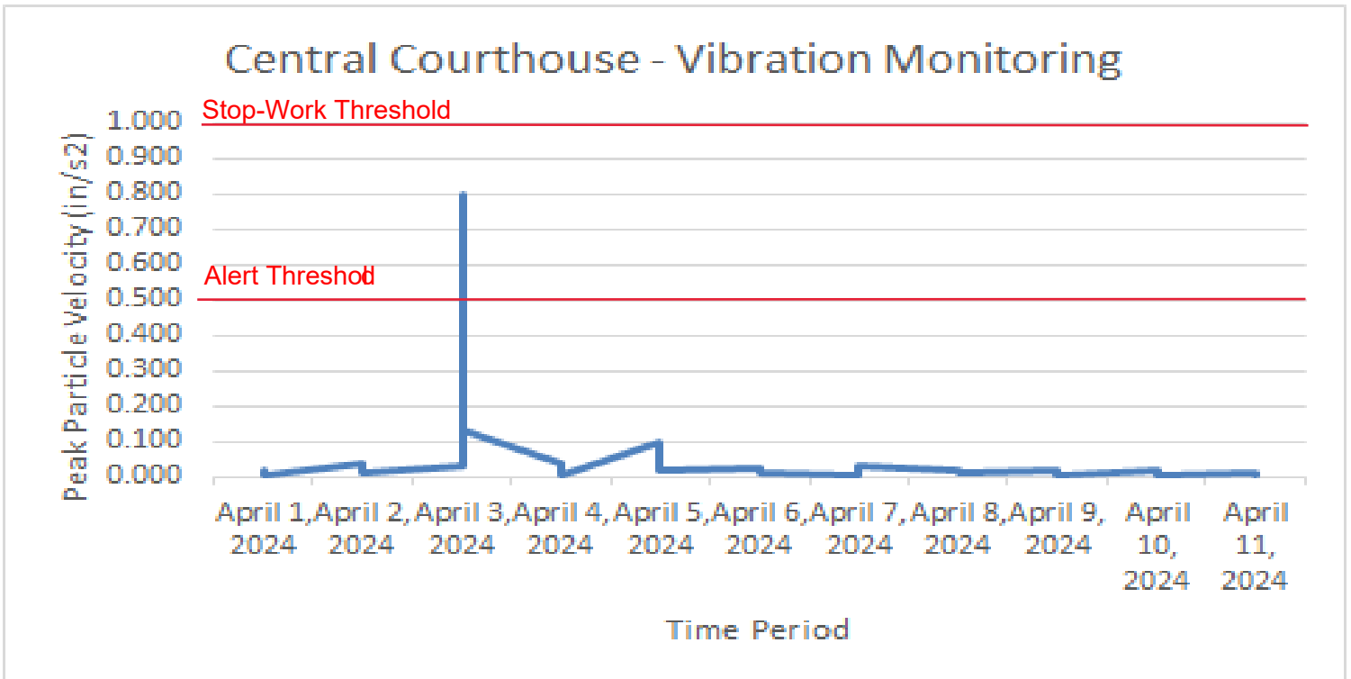
Central Courthouse Vibration Monitor – VM-01 – April 2024:
