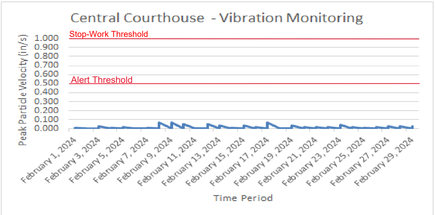
Central Courthouse Vibration Monitor – VM-01 – February 2024:
