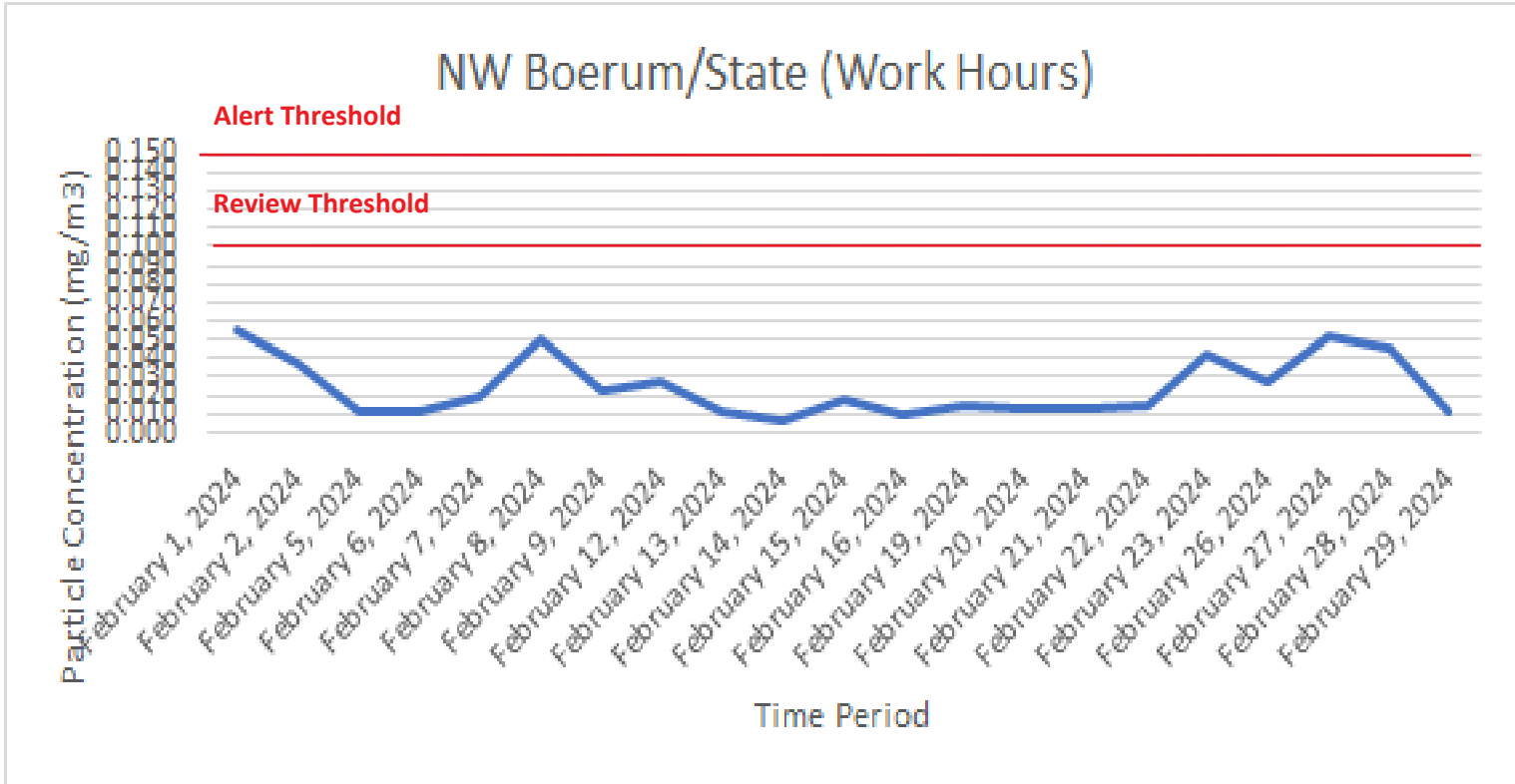
Dust Monitoring Unit – NW Corner – February 2024:
