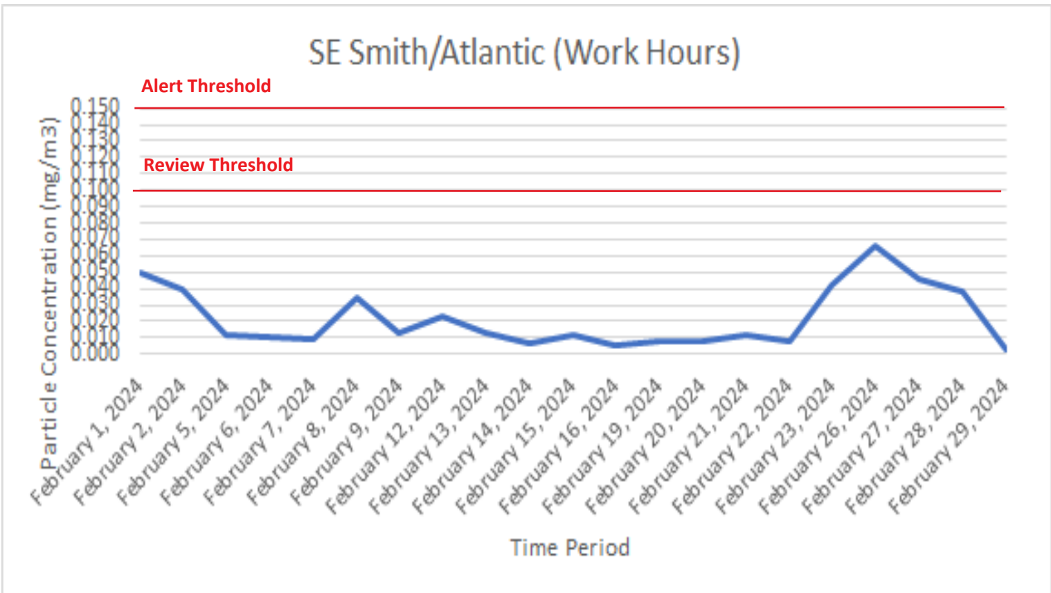
Dust Monitoring Unit – SE Corner – February 2024:
